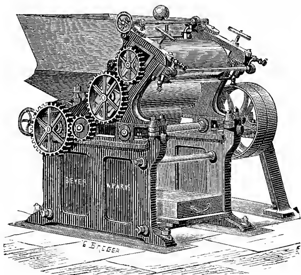
BRUNOT'S POUNDING-MACHINE.
